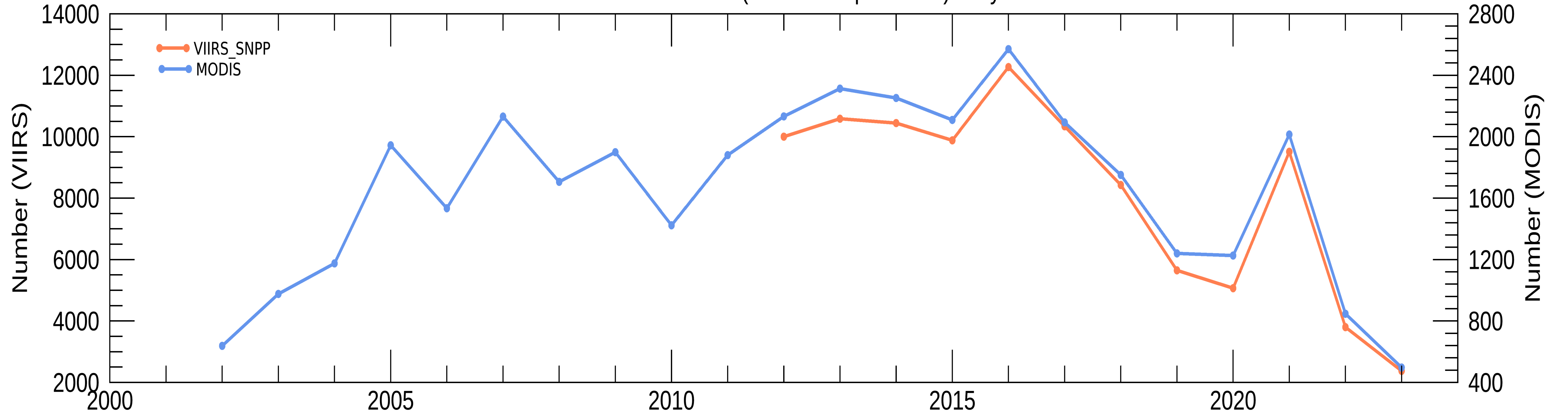
Fire Detection Counts (Total for Sep. to Nov.) Haryana
